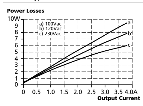
Fig. 8-2 Losses vs. output current at 24V, typ.
