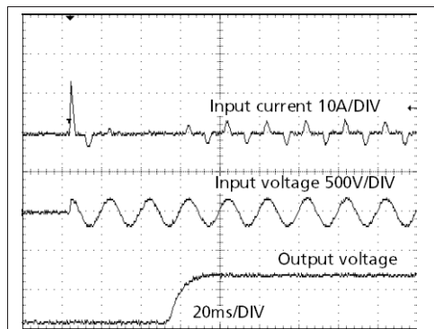
Fig. 5-3 Typical turn-on behavior at 120Vac and 25°C ambient
